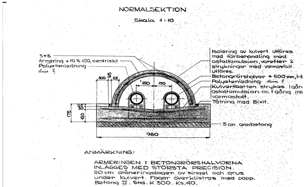
Figure 2. Cross-section of a typical non-viable half culvert.
