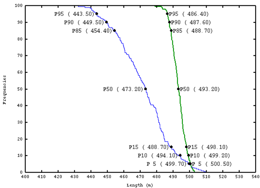
Figure11: Global estimation of pipe length above the threshold ignoring dose rate values (in blue) and including them (in green). Inverse cumulative representation.
