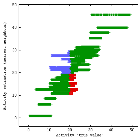
Figure 9: Comparison between deterministic estimation and true value and misclassification errors in blue (false positive) and in red (false negative).
