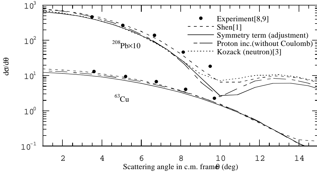
Fig.3 Neutron-incident differential cross section at T=155MeV
