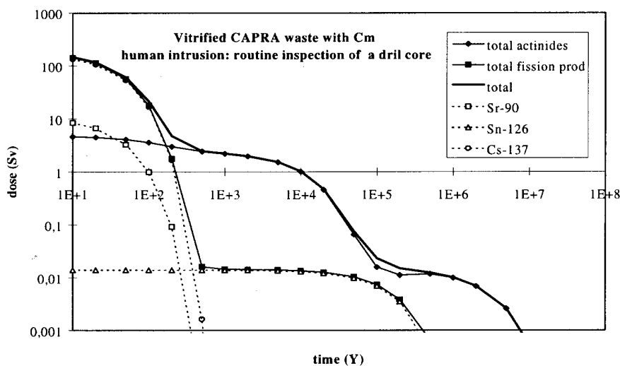
Figure 1. Dose from the core examination scenario for vitrified HLW from reprocessing of CAPRA fuel
